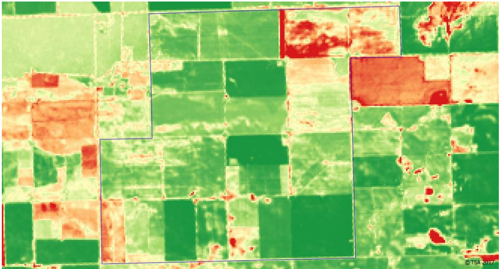
NDVI 21-1-2017
